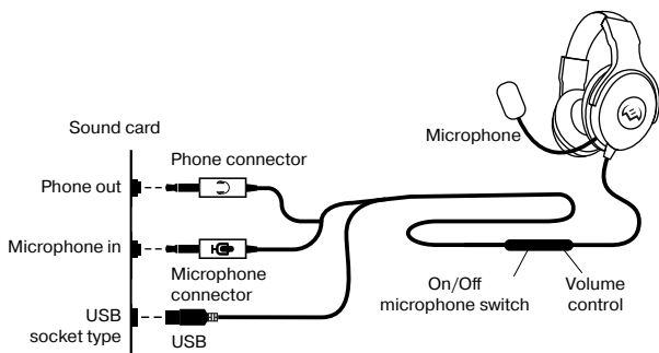
Fig. 1. Connection diagram
